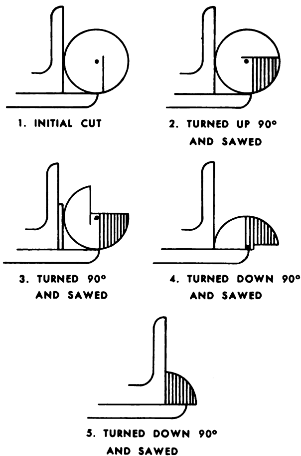
Figure 9-2. Sawing oversized logs.
